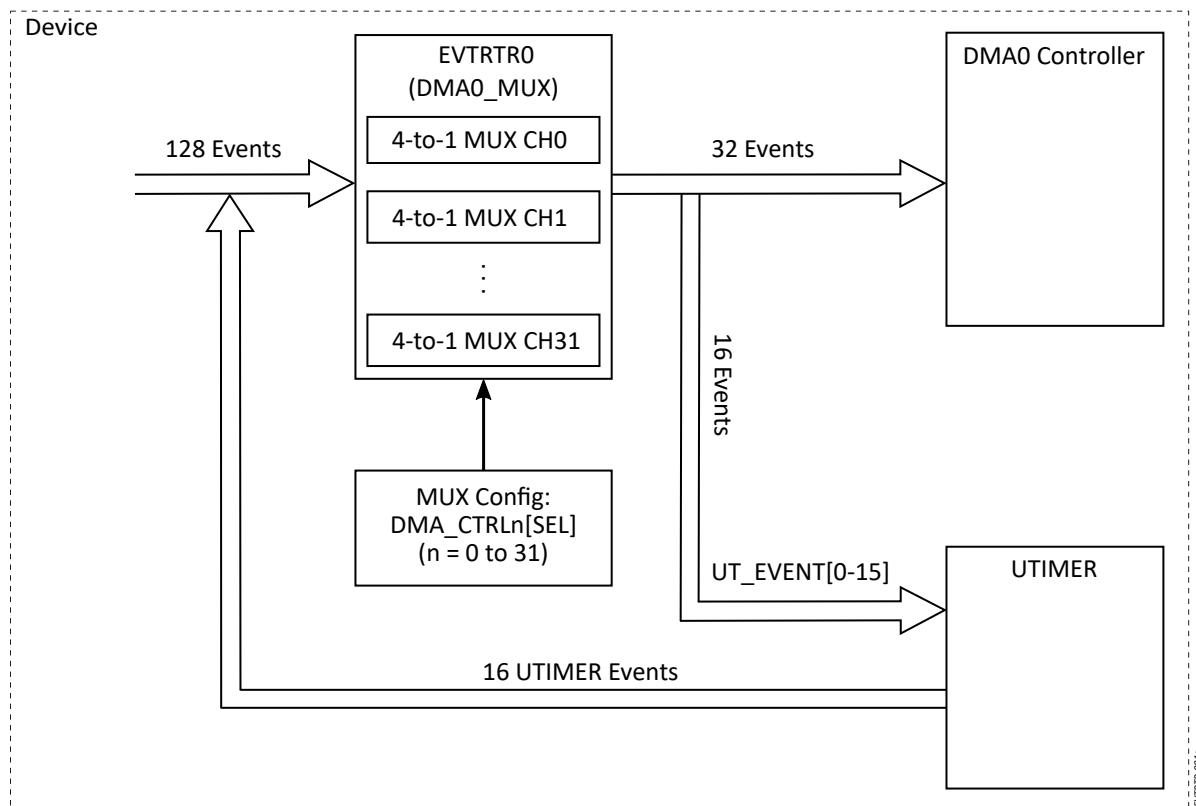
Figure 3-9 EVTRTR Overview
